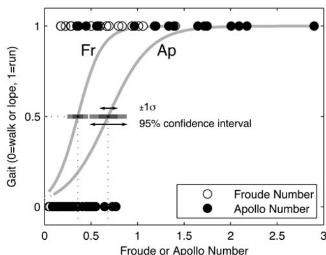
Figure 4. Gait transition probability as a function of Froude and Apollo numbers. Transition probability curves P(Fr) and P(Ap) for the binary variable gait (walk/lope=0, run=1). Here, P(x) = 1/(1 + \exp[-(\alpha + \beta x)]) , with the transition defined by P(x) = 1/2 , where x = -\alpha/\beta (Text S1). For values of (\alpha, \beta) see Table 3. doi:10.1371/journal.pone.0006614.g004
